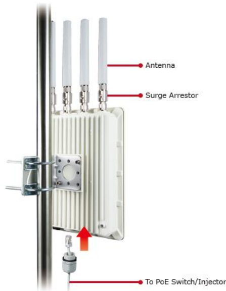
Figure 3-5 Attach the surge arrestors, antenna and PoE cable
