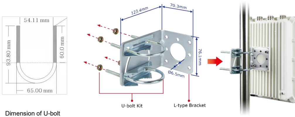
Figure 3-4 Mounting on the cylinder
