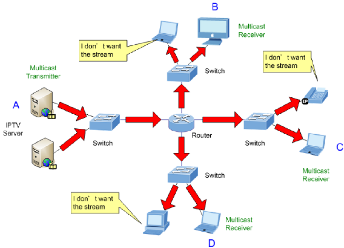
Figure 4-8-2: Multicast Flooding
