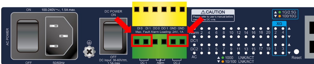
Figure 2-1-5-1: MGSW-24160F DC power input
