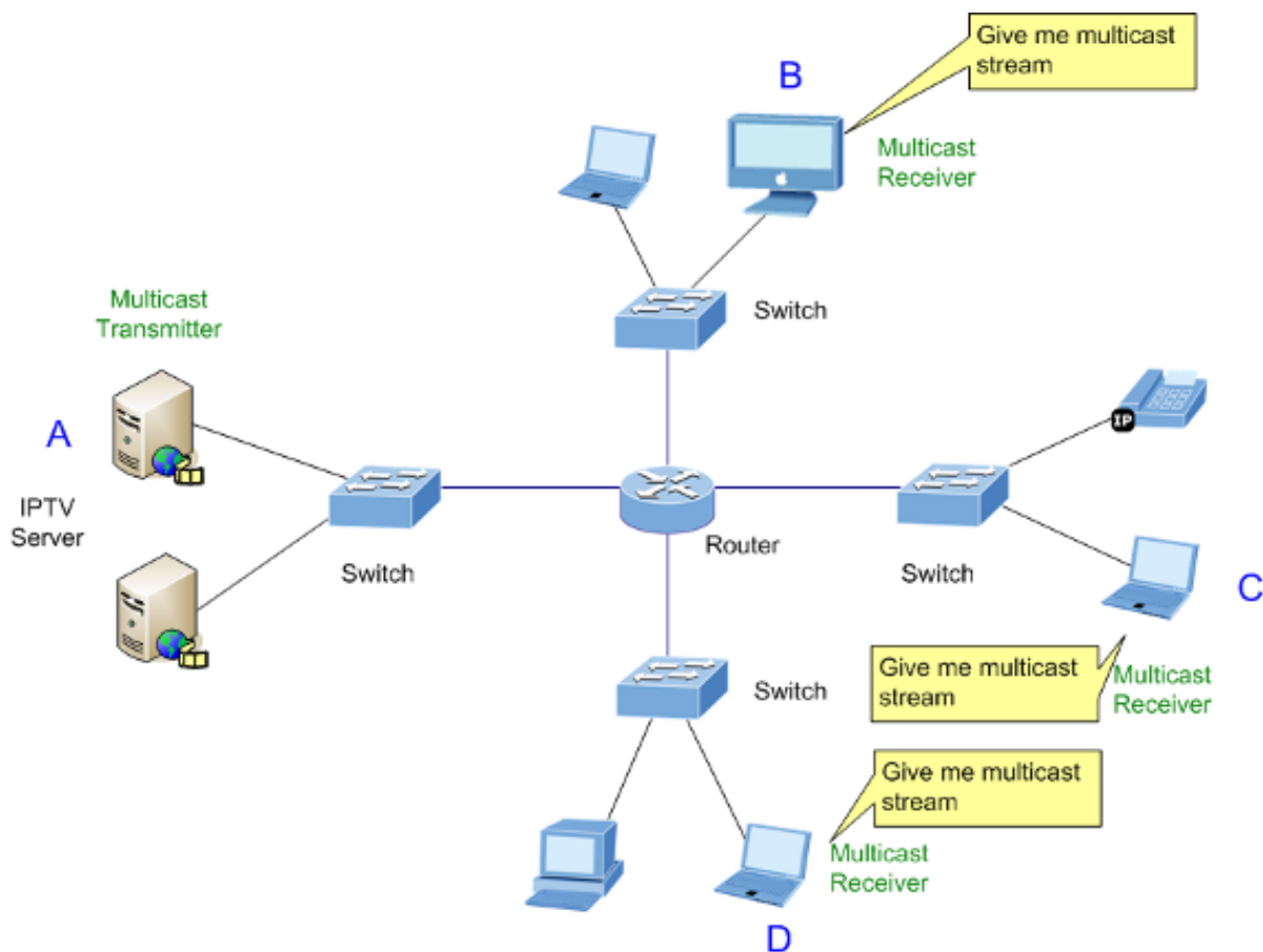
Figure 4-8-1: Multicast Service
