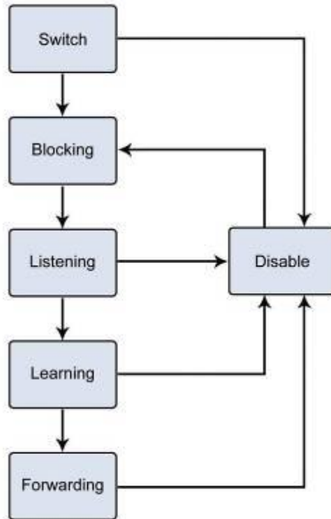
Figure 4-6-1-1: STP Port State Transitions
