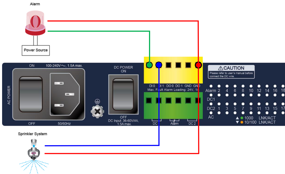
Figure 2-1-7-4 Wiring DO0 and DO1 to Open Detector
