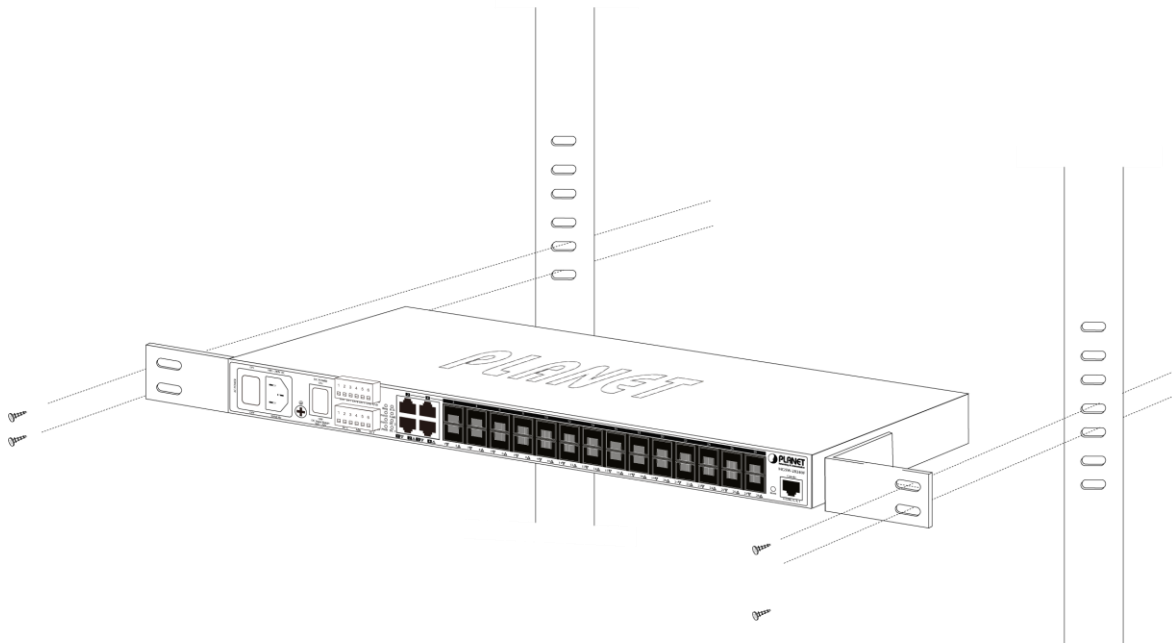
Figure 2-2-2-1 Mounting the Managed Metro Switch on a Rack
