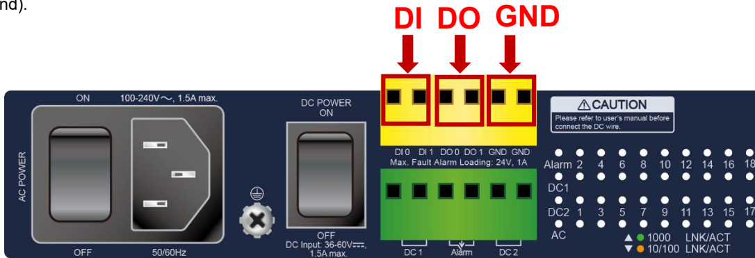
Figure 2-1-7-1 Wiring Digital Inputs/Outputs
