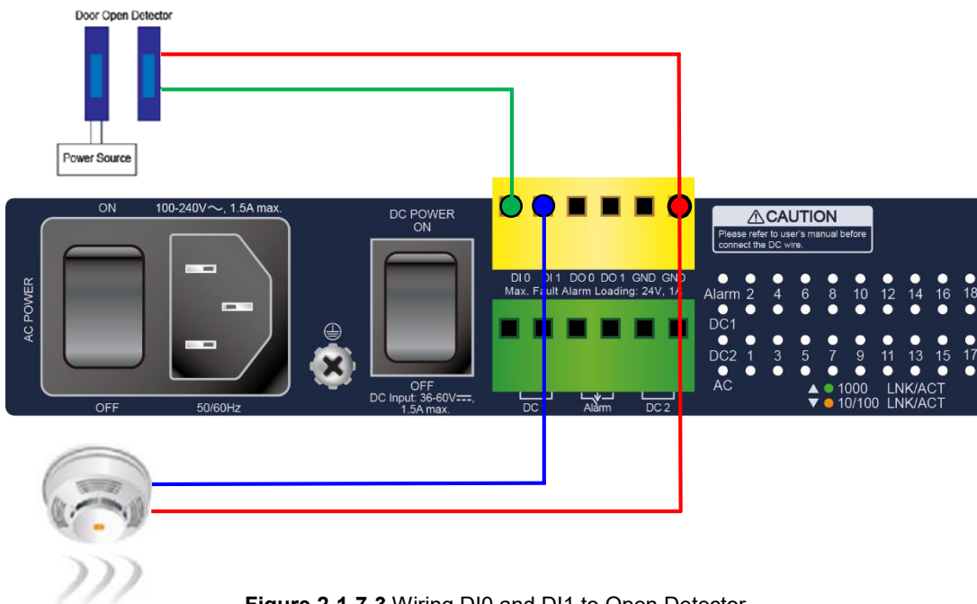
Figure 2-1-7-3 Wiring DI0 and DI1 to Open Detector
