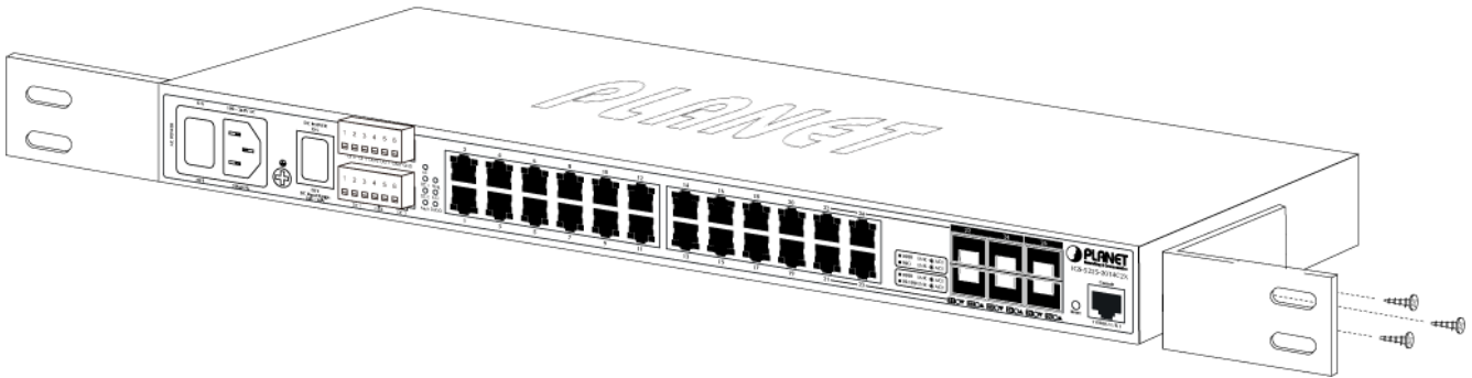
Figure 2-2-2-1 Attach Brackets to the Managed Metro Switch.
