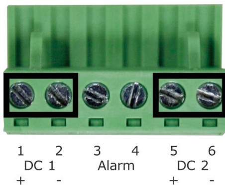
Figure 2-1-5-2 6-pin Terminal Block Power Wiring Input for MGSW-24160F
