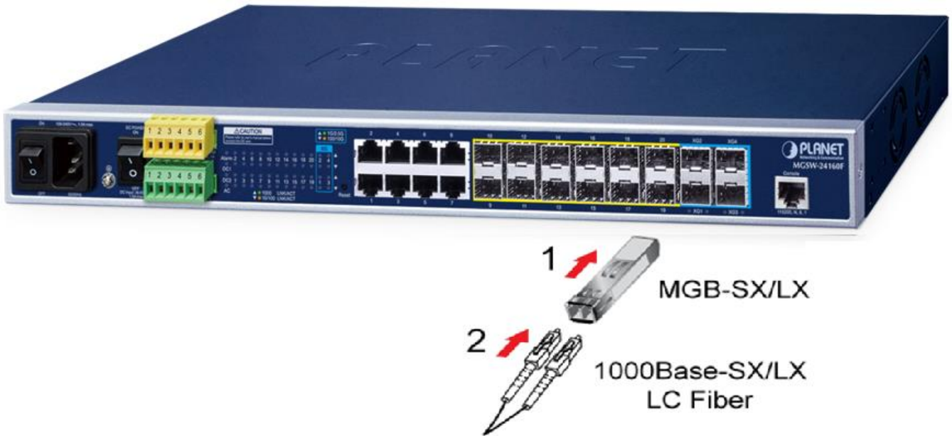
Figure 2-3-1-1: Plug in the SFP/SFP+ Transceiver
