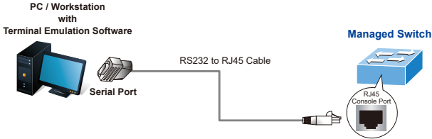
Figure 4-1: Managed Switch Console Connectivity
