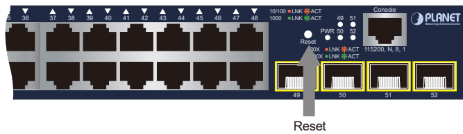
Figure 5-9: GS-4210-48T4S Reset Button
