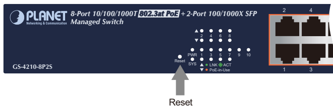
Figure 5-3: GS-4210-8P2S Reset Button
