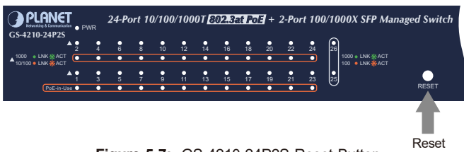
Figure 5-7: GS-4210-24P2S Reset Button
