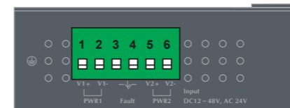
Figure 2-3: Industrial Fast Ethernet Switch Upper Panel
