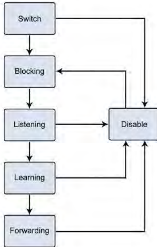
Figure 4-3-4-1: STP Port State Transitions
