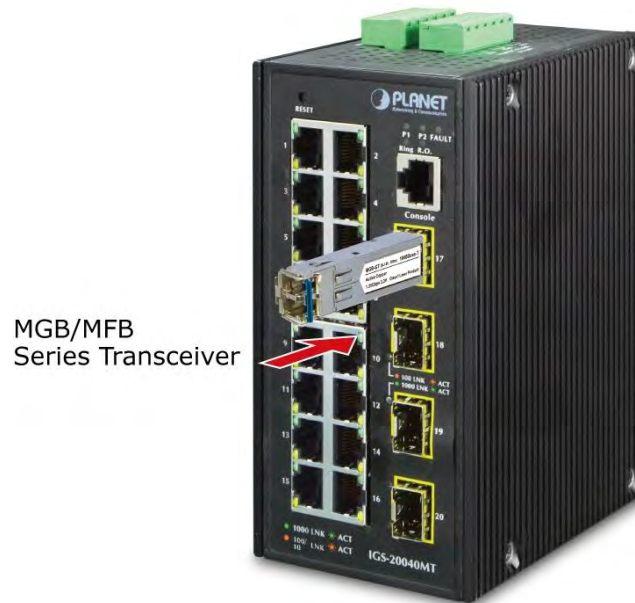
Figure 2-17: Plugging in the SFP/SFP+ Transceiver
