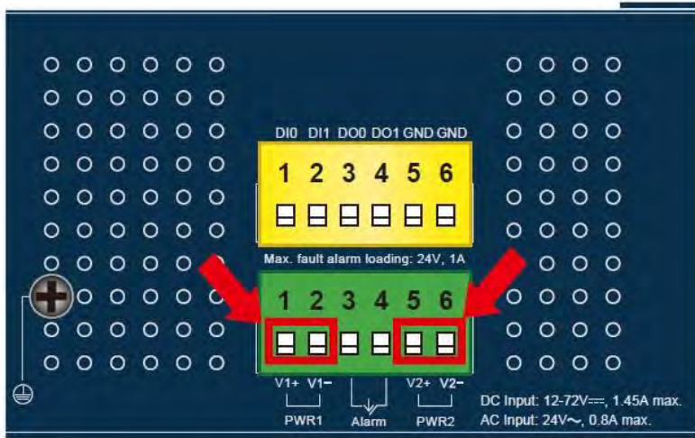
Figure 2-11: IGS-12040MT Upper Panel
