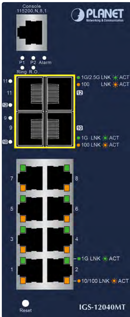
Figure 2-3: IGS-12040MT Switch Front Panel
