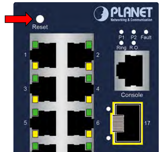
Figure 2-8: IGS-20040MT Reset Button
