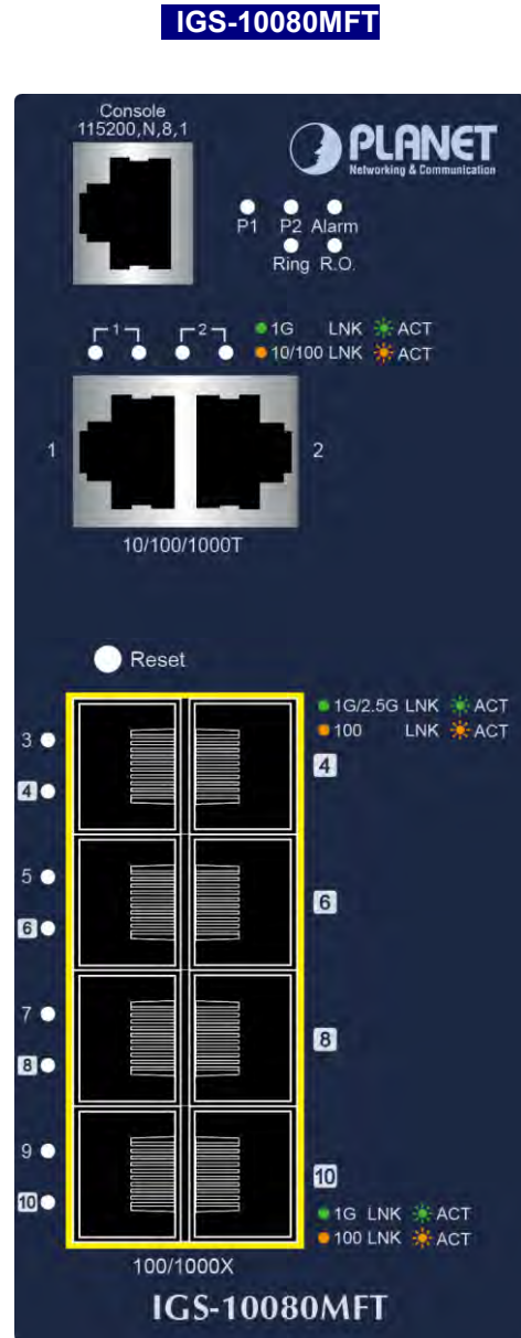
Figure 2-2: IGS-10080MFT Switch Front Panel
