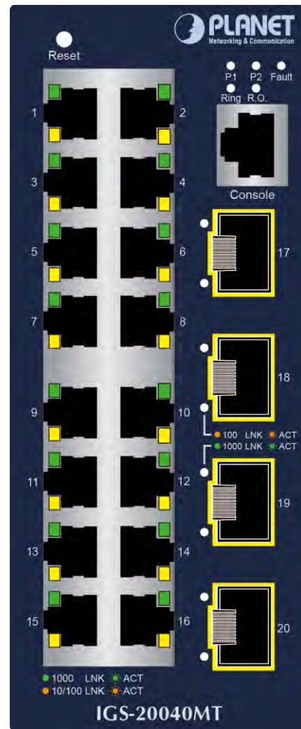
Figure 2-4: IGS-20040MT Switch Front Panel
