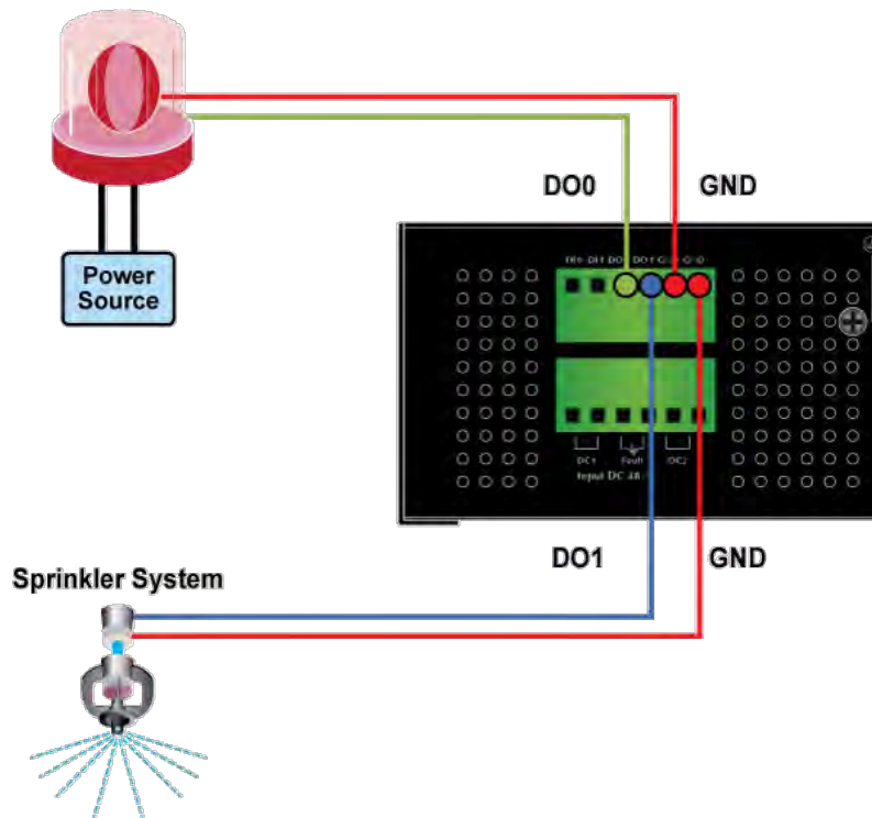
Figure 2-16: Wiring DO0 and DO1 to Open Detector
