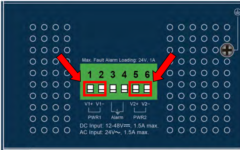
Figure 2-10: IGS-10080MFT Upper Panel
