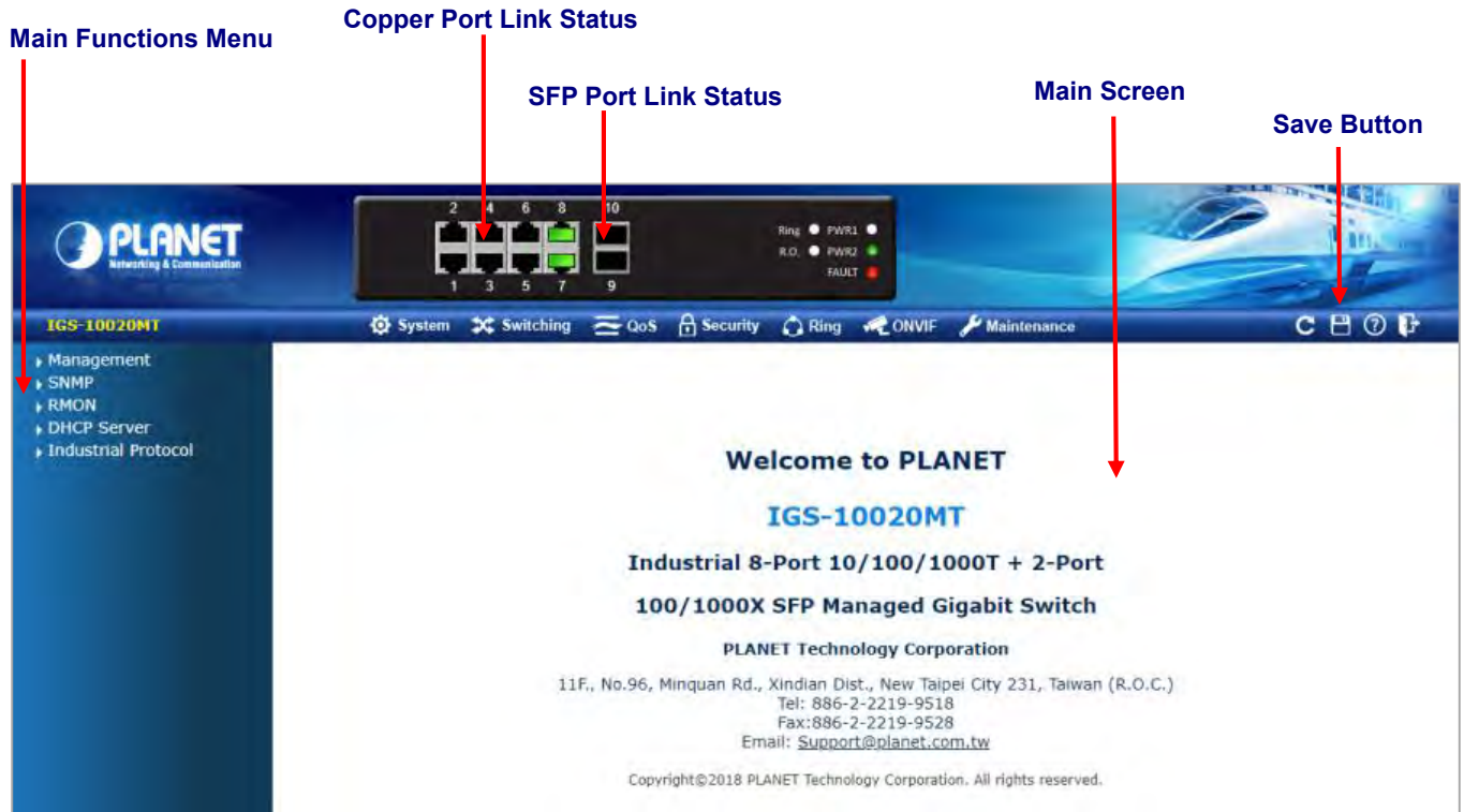
Figure 4-1-4: Main page
