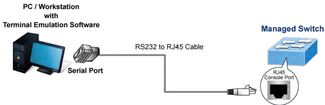
Figure 3-1: Industrial L2+ Managed Switch Console Connectivity
