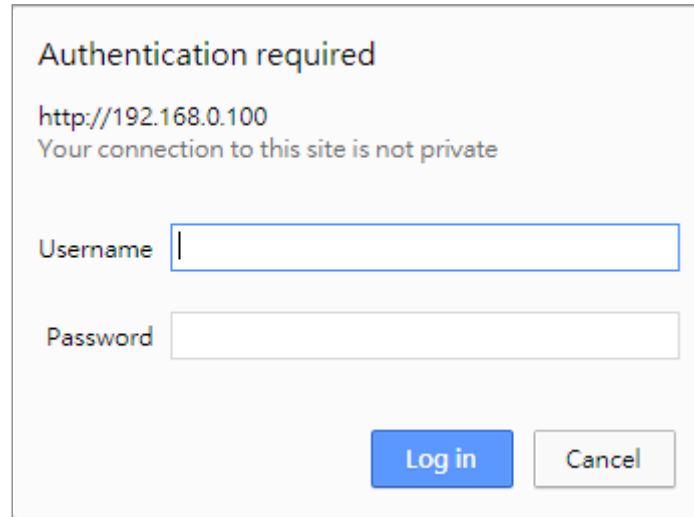
Figure 4-1-2: Login Screen
