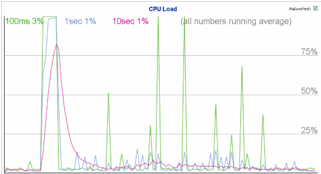
Figure 4-2-14: CPU Load Screenshot
