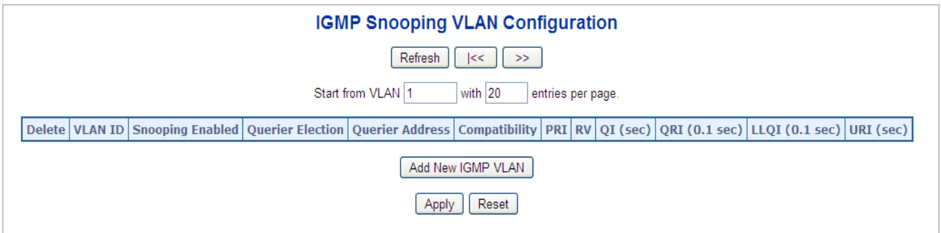
Figure 4-8-8: IGMP Snooping VLAN Configuration Screenshot
