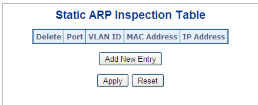
Figure 4-12-14: Static ARP Inspection Table Screen Screenshot
