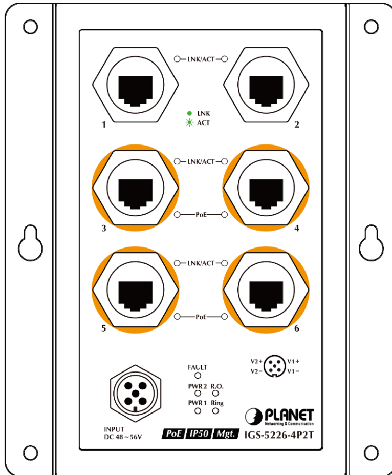
Figure 2-2: IGS-5226-4P2T LED on Front Panel
