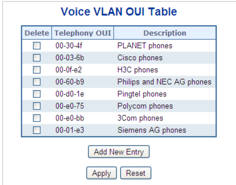
Figure 4-9-18: Voice VLAN OUI Table Screenshot
