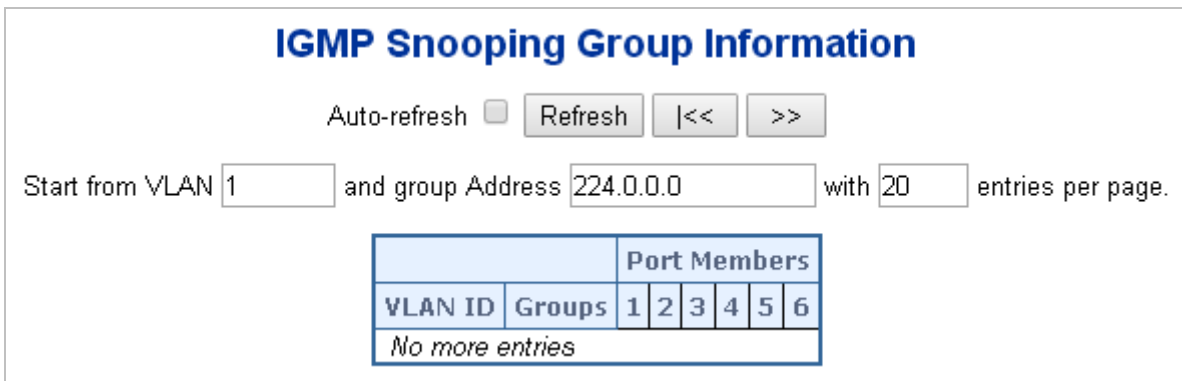
Figure 4-8-11: IGMP Snooping Groups Information Screenshot
