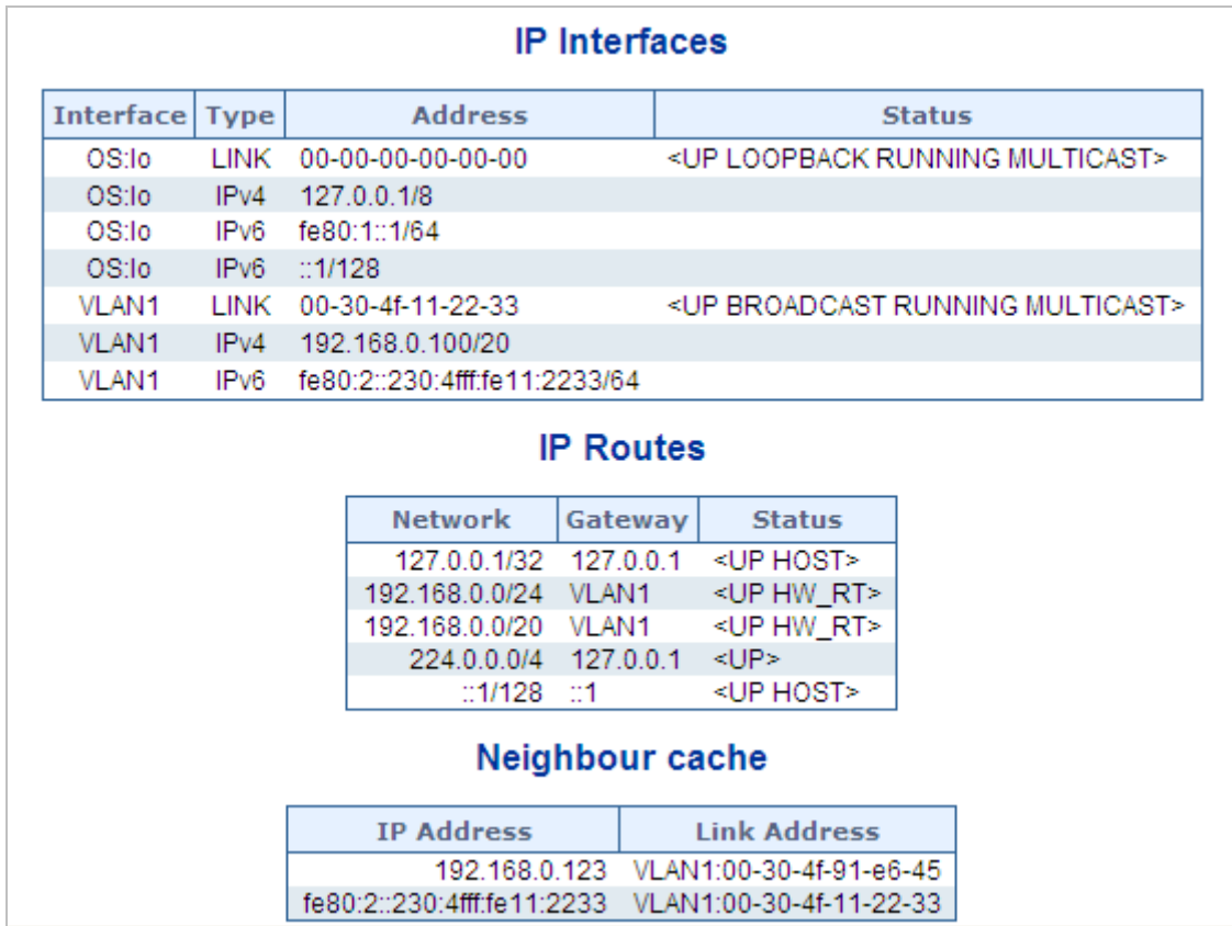
Figure 4-2-3: IP Status Screenshot
