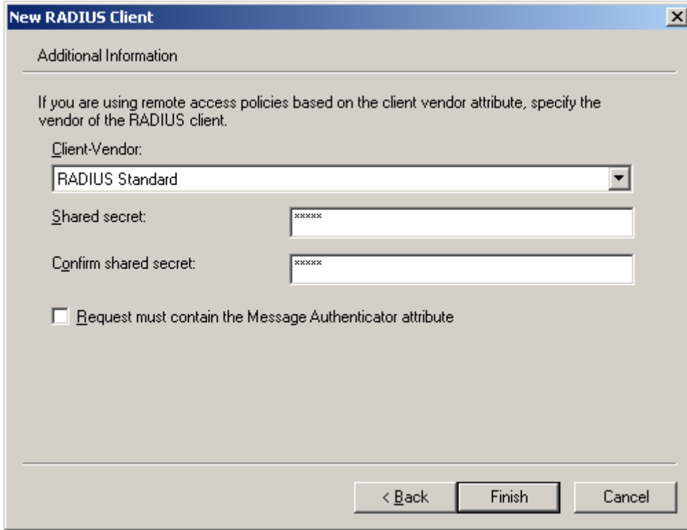
Figure 4-11-14: Windows Server RADIUS Server Setting
