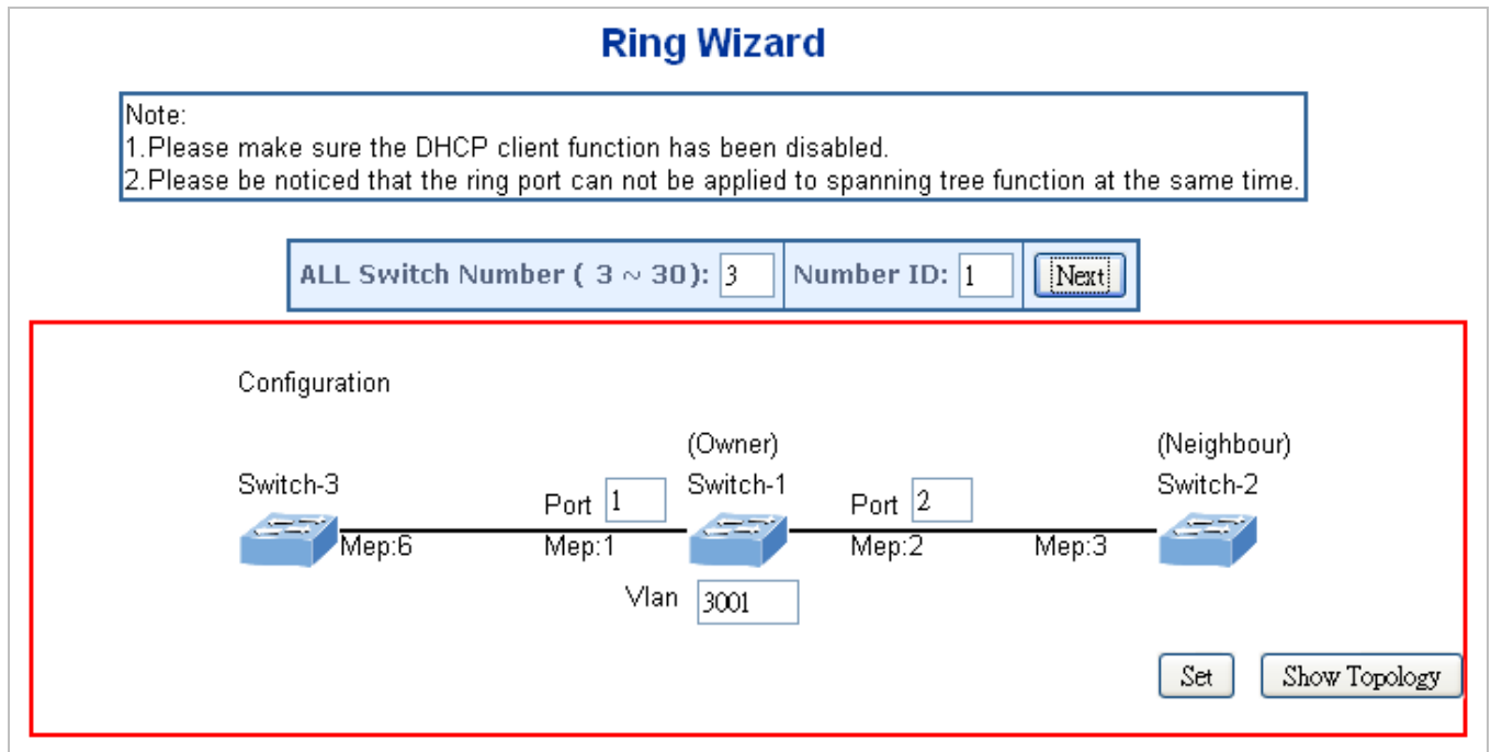
Figure 4-20-5: Ring Wizard Screenshot
