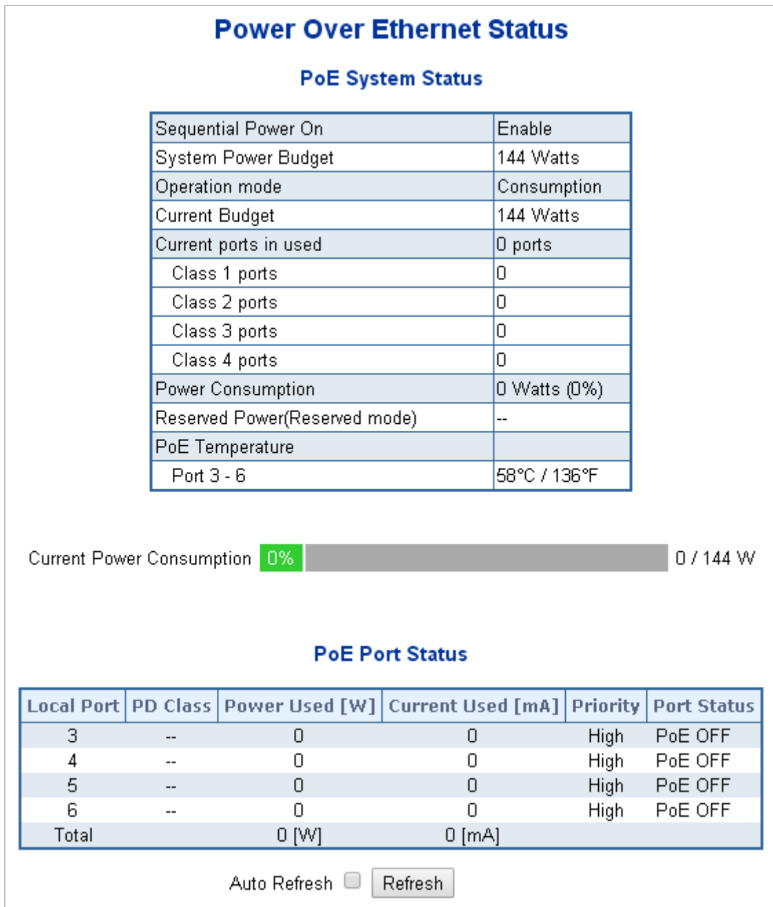
Figure 4-16-5: PoE Status Screenshot
