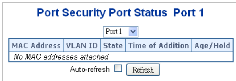
Figure 4-12-7: Port Security Detail Screen Screenshot
