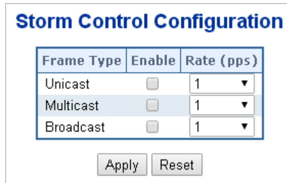
Figure 4-9-15: Storm Control Configuration Screenshot
