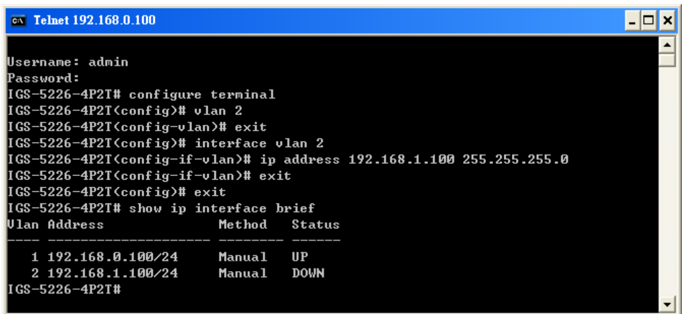
Figure 3-1: Remote Telnet Interface Main Screen of Industrial Managed Switch
