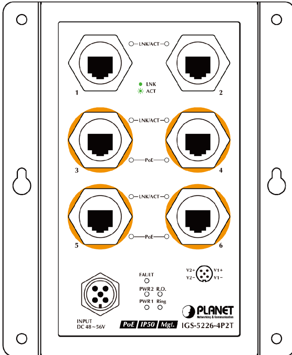
Figure 2-1: IGS-5226-4P2T Switch Front Panel
