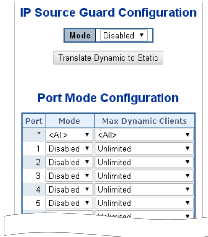
Figure 4-12-10: IP Source Guard Configuration Screen Screenshot
