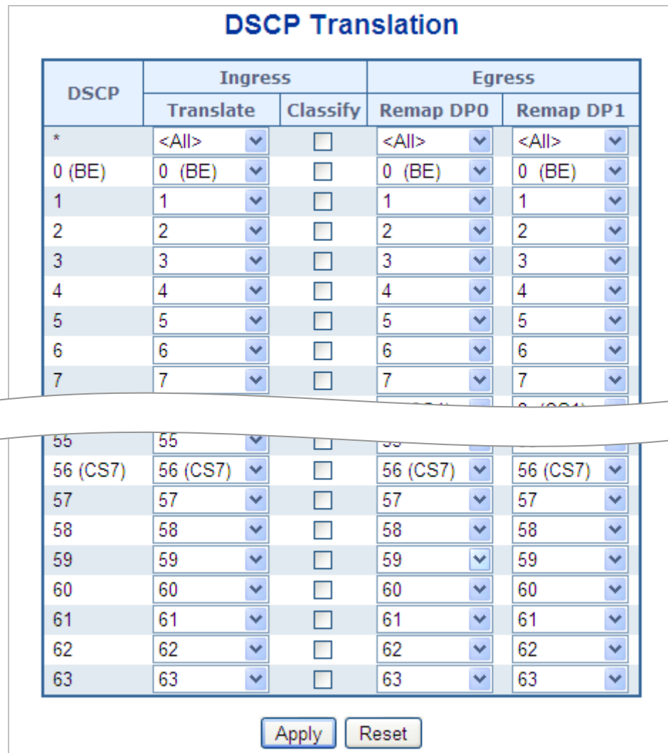
Figure 4-9-10: DSCP Translation Screenshot
