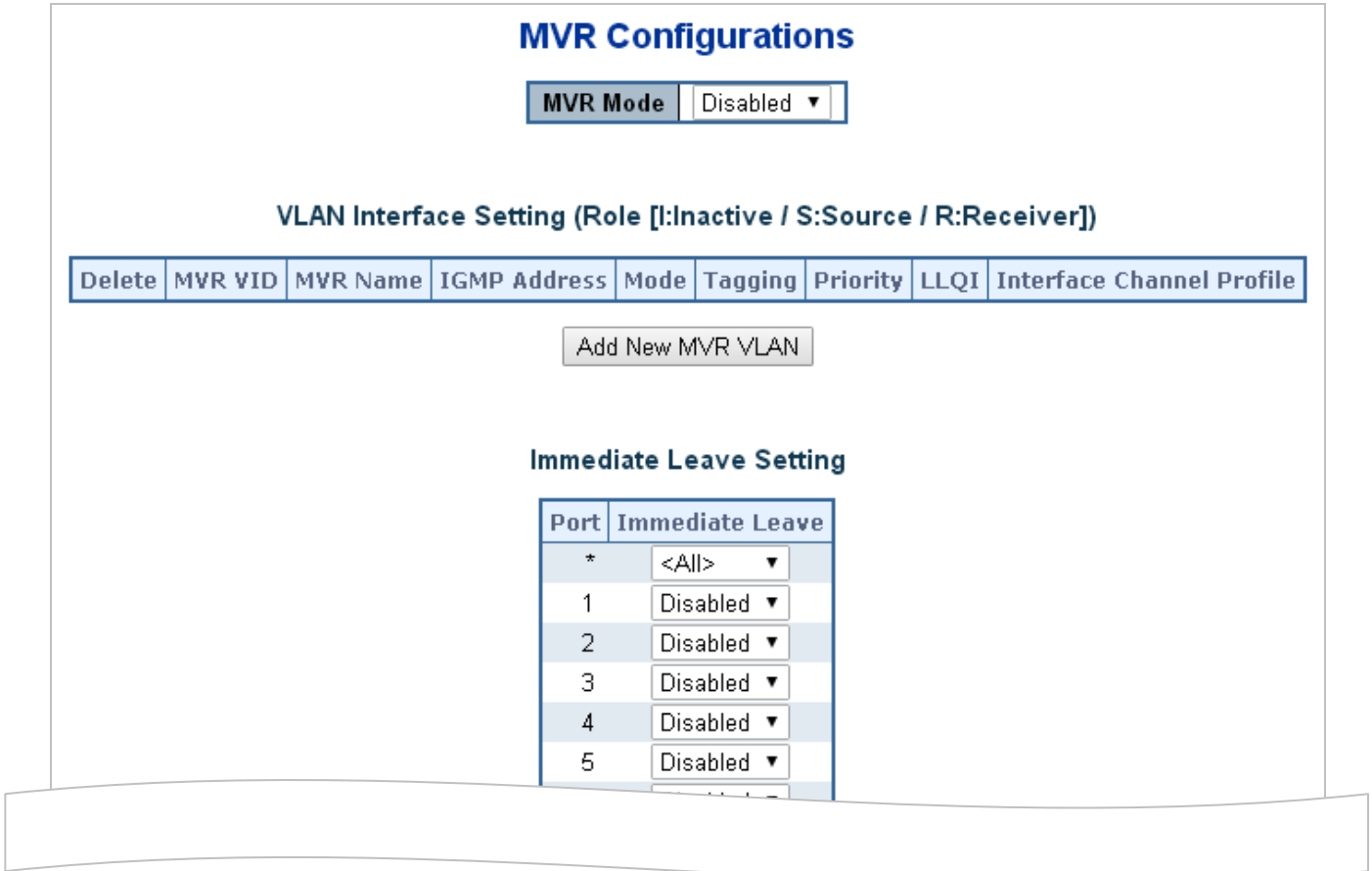
Figure 4-8-19: MVR Configuration Screenshot
