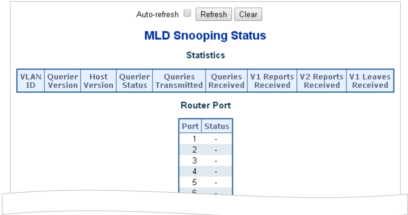
Figure 4-8-16: MLD Snooping Status Screenshot
