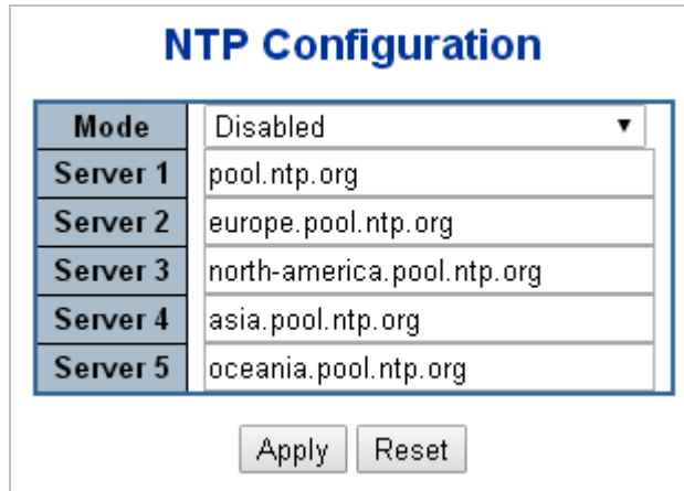
Figure 4-2-8: NTP Configuration Screenshot
