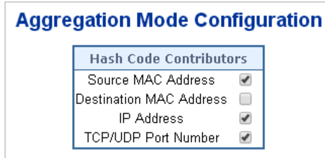
Figure 4-5-2 : Aggregation Mode Configuration Screenshot
