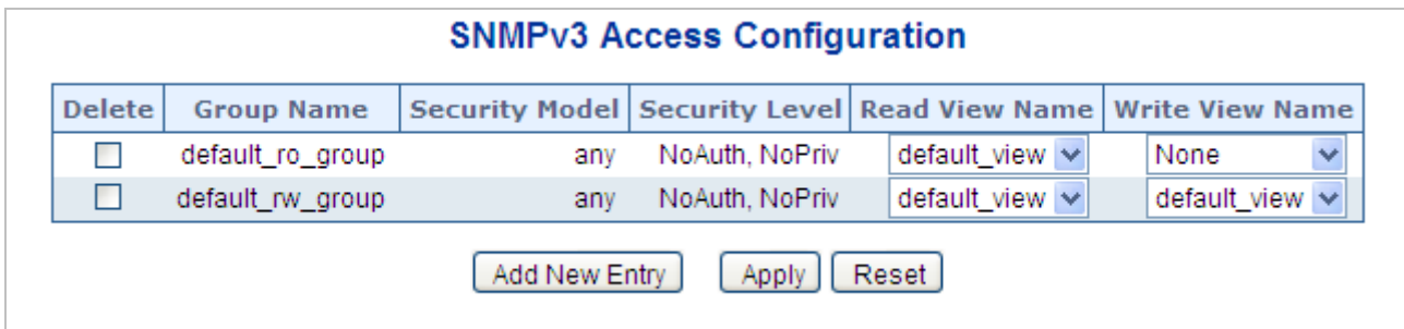
Figure 4-3-8: SNMPv3 Accesses Configuration Screenshot
