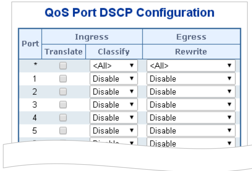
Figure 4-9-8: QoS Port DSCP Configuration Screenshot
