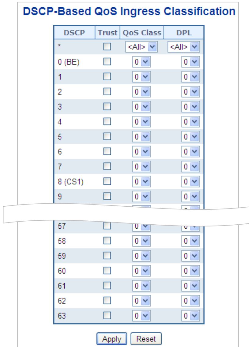
Figure 4-9-9: DSCP-based QoS Ingress Classification Screenshot
