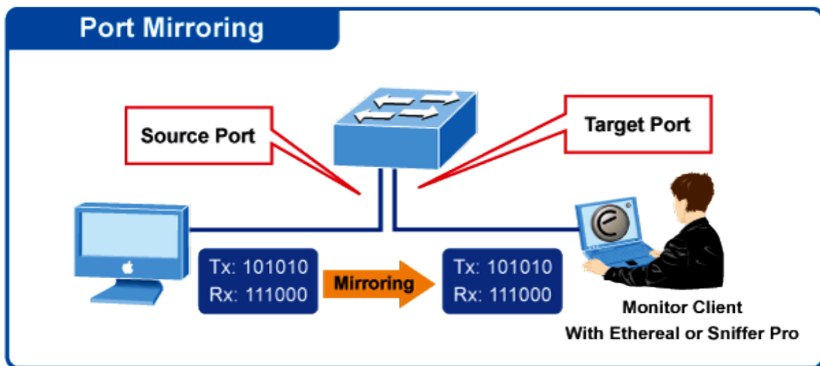
Figure 4-4-4: Port Mirror Application
