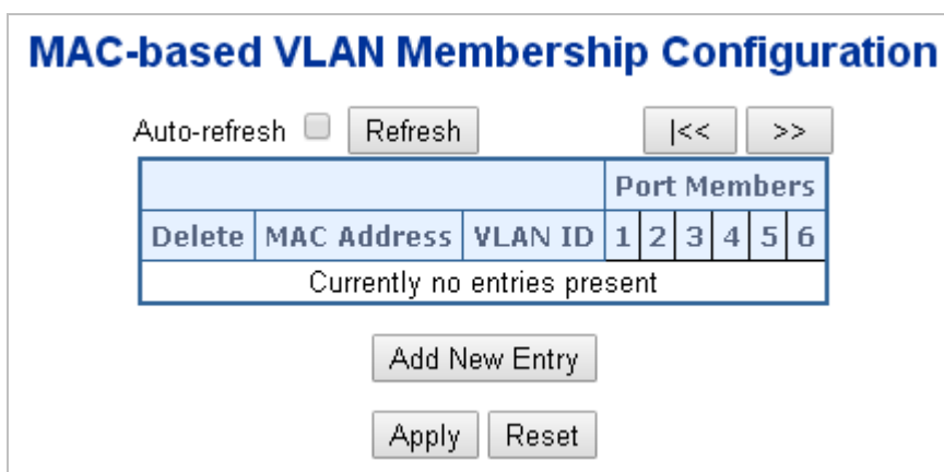
Figure 4-6-18: MAC-based VLAN Membership Configuration Screenshot
