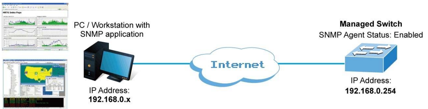
Figure 3-4: SNMP Management
