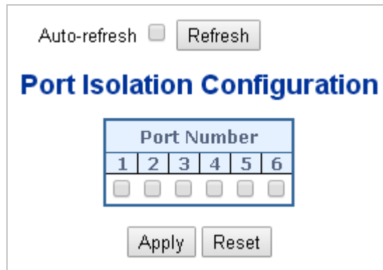
Figure 4-6-7: Port Isolation Configuration Screenshot
