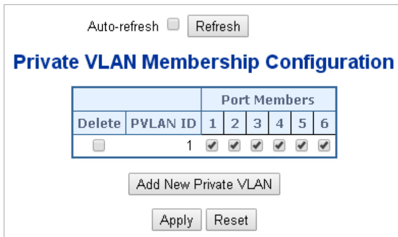
Figure 4-6-6 Private VLAN Membership Configuration screenshot
