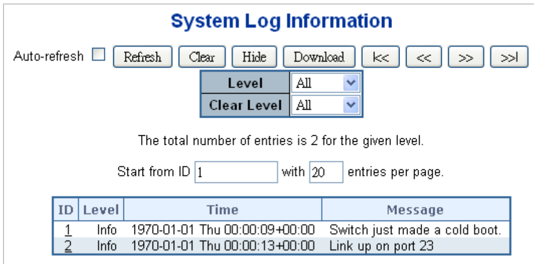
Figure 4-2-15: System Log Screenshot
