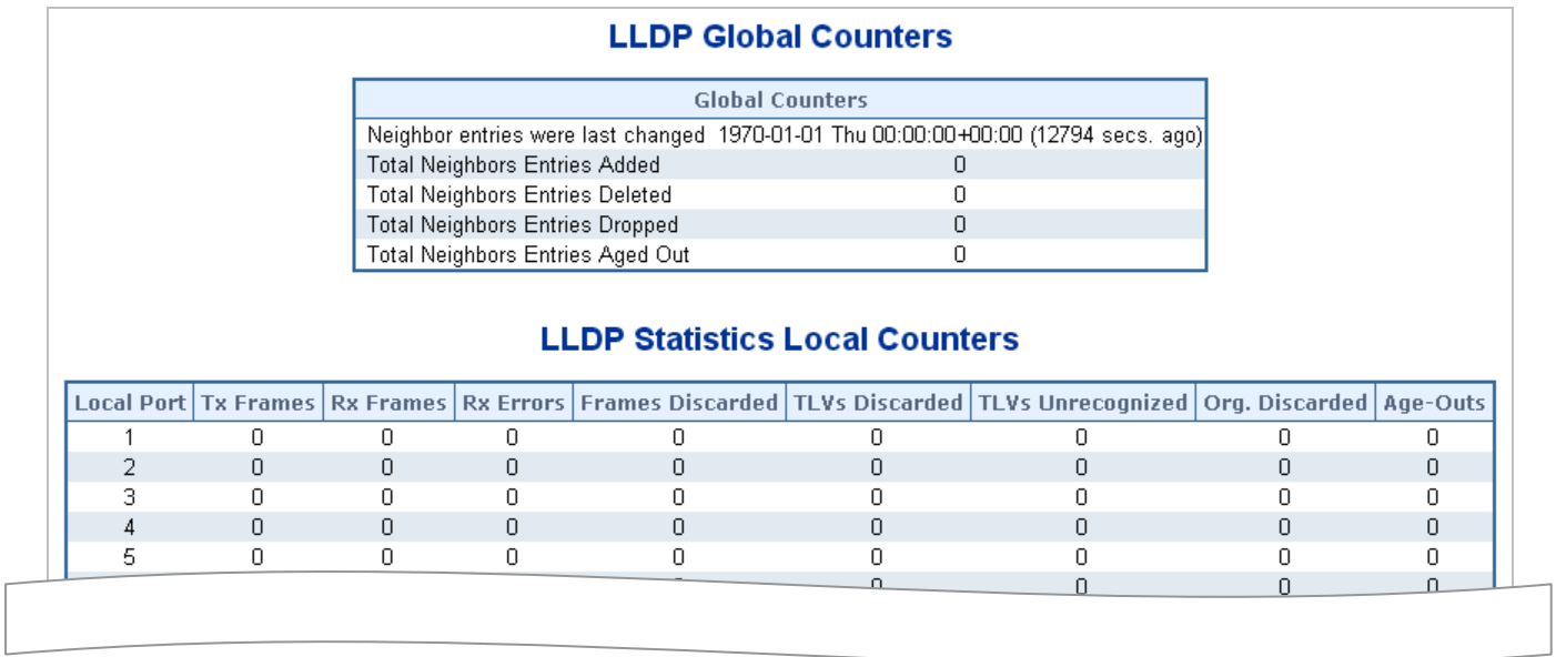
Figure 4-14-5: LLDP Statistics Screenshot
