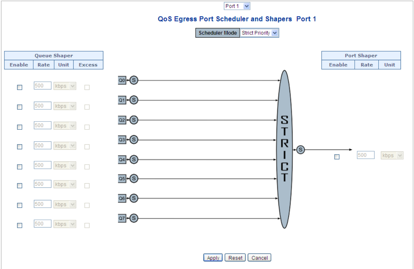
Figure 4-9-5: QoS Egress Port Schedule and Shapers Screenshot
