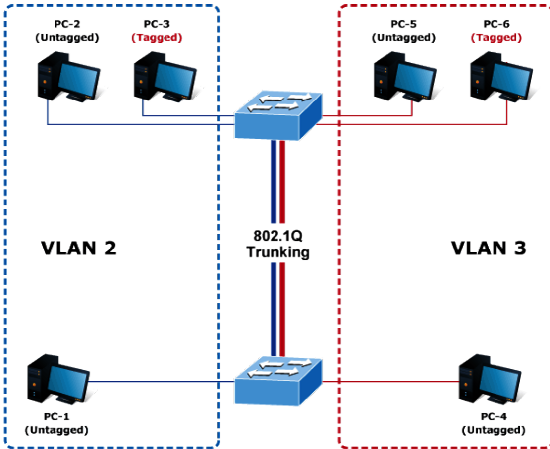
Figure 4-6-12: VLAN Trunking Diagram
