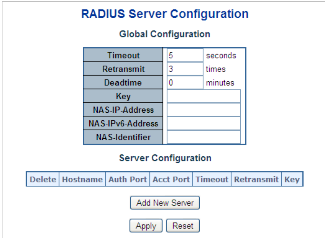
Figure 4-11-7: RADIUS Server Configuration Screenshot
