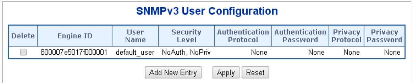
Figure 4-3-5: SNMPv3 Users Configuration Screenshot
