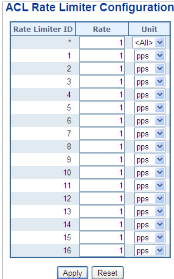
Figure 4-10-5: ACL Rate Limiter Configuration Screenshot
