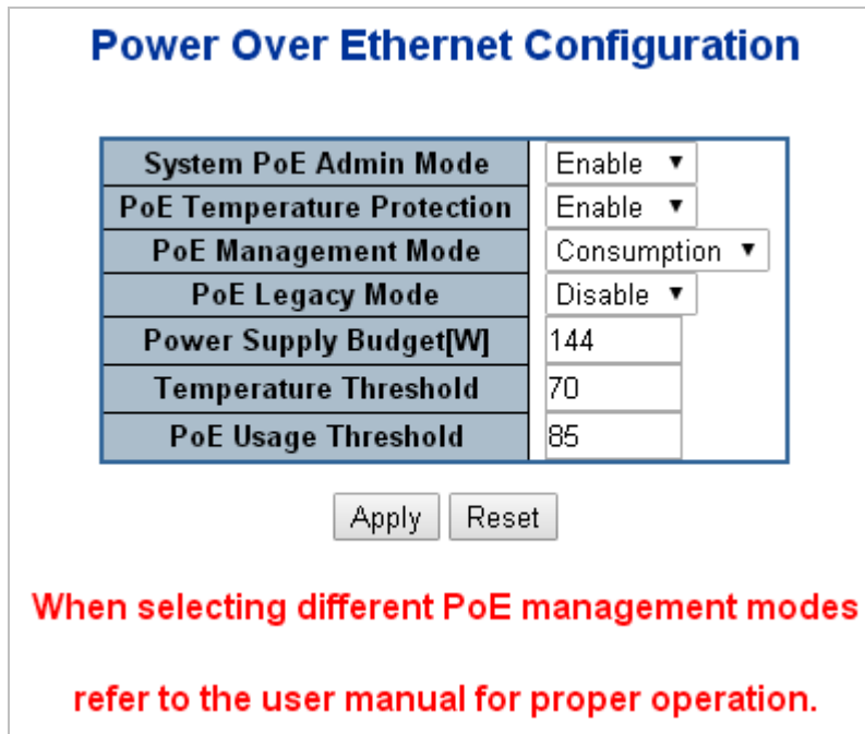
Figure 4-16-2: PoE Configuration Screenshot
