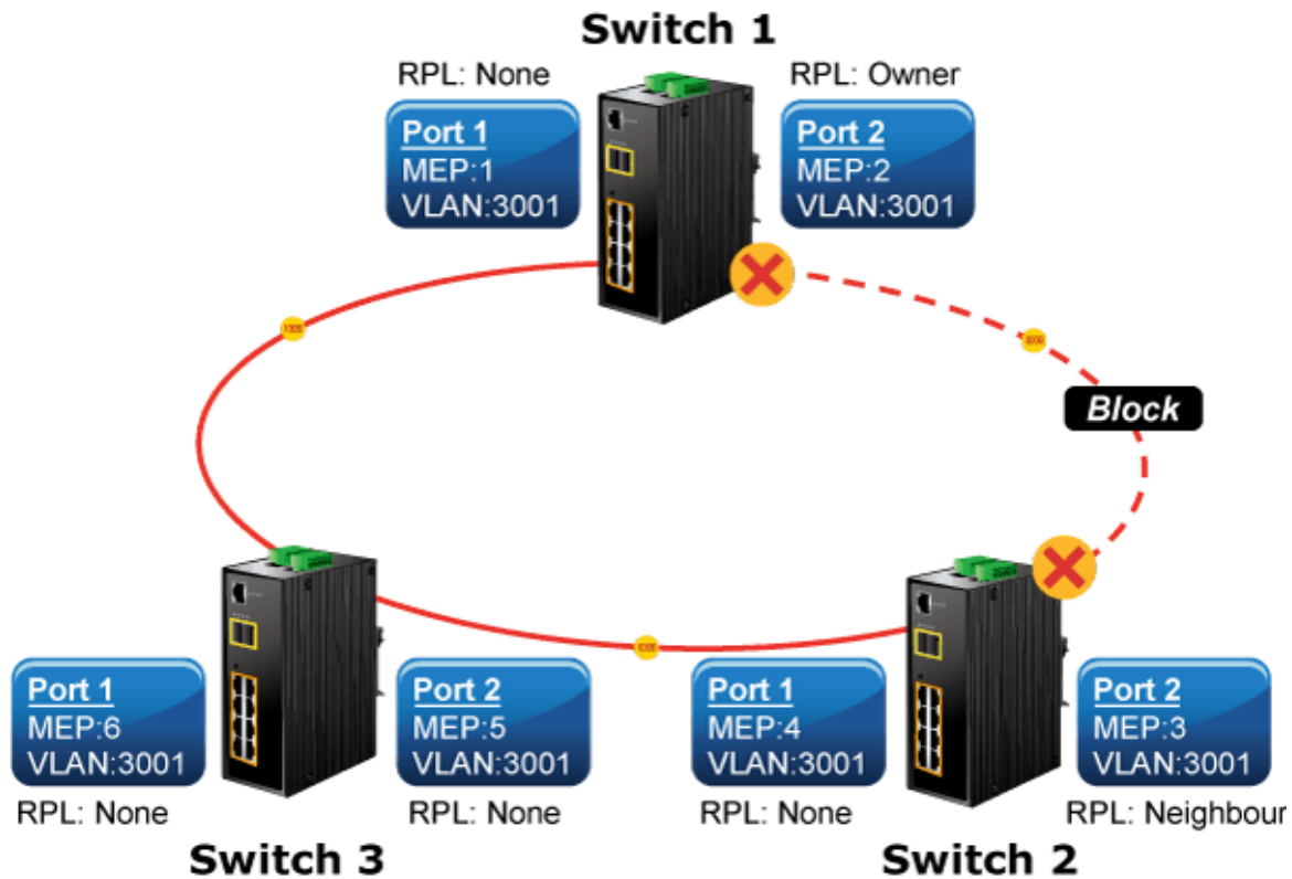
Figure 4-20-6: Ring Example Diagram
