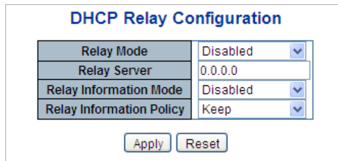
Figure 4-2-12 DHCP Relay Configuration Screenshot
