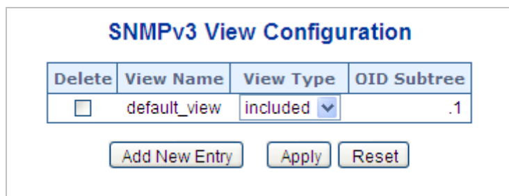
Figure 4-3-7: SNMPv3 Views Configuration Screenshot
