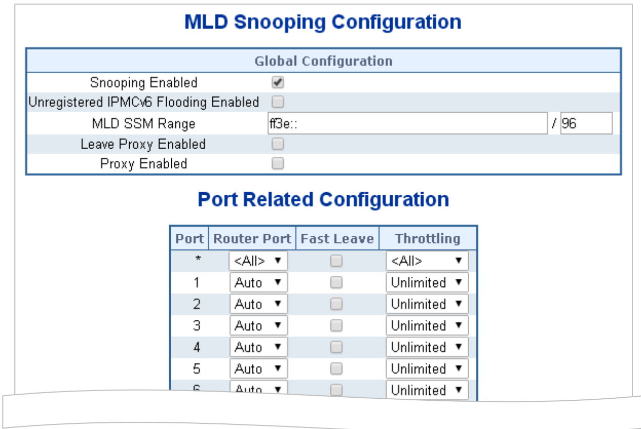
Figure 4-8-13: MLD Snooping Configuration Screenshot
