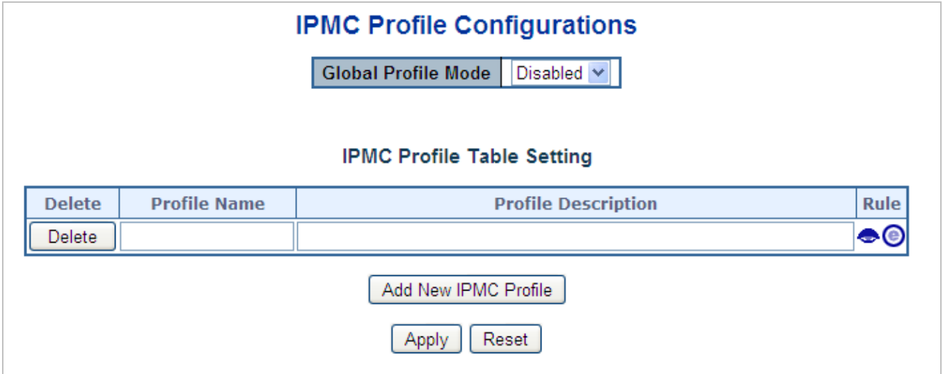
Figure 4-8-5: IPMC Profile Configuration Screenshot
