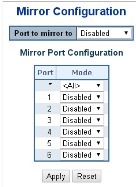
Figure 4-4-5: Mirror Configuration Screenshot
