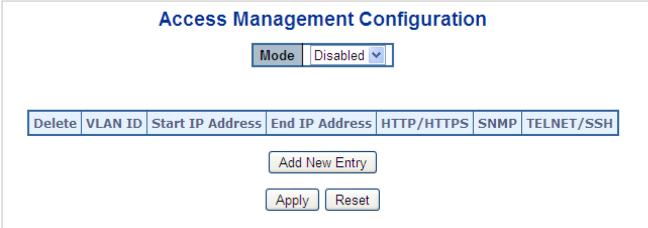
Figure 4-12-2: Access Management Configuration Overview Screenshot
