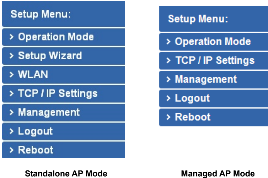
Figure 5-1 Main Menu
