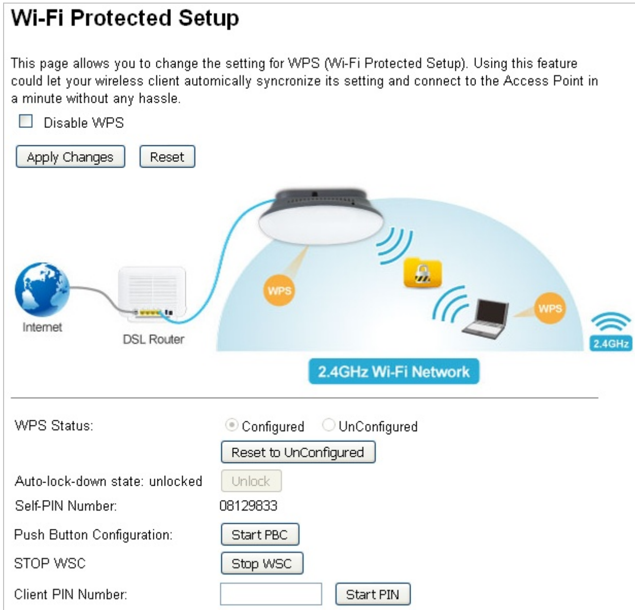
Figure 5-38 WPS
