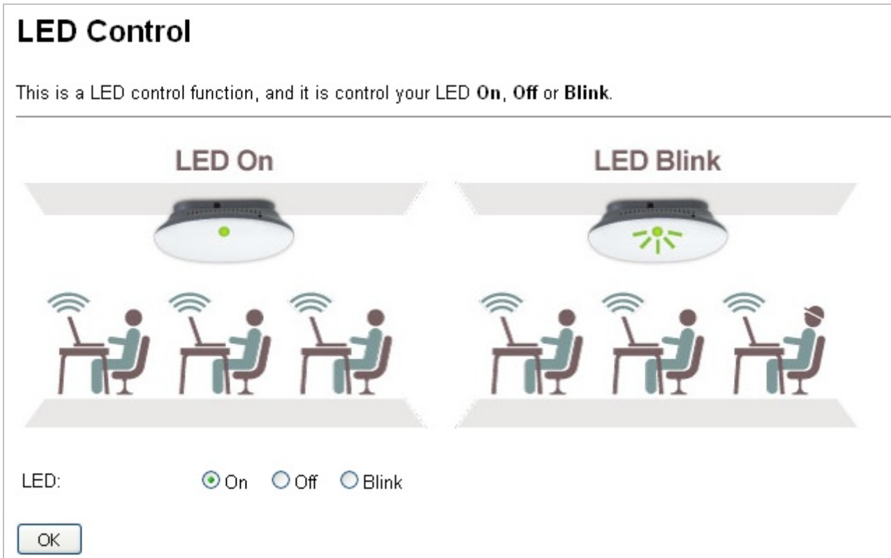
Figure 5-56 LED Control
