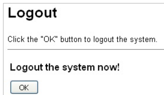
Figure 5-57 Logout
