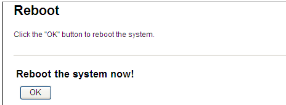
Figure 5-58 Reboot
