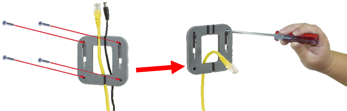
Figure 3-1 WNAP-C3220A Installation Diagram 1
