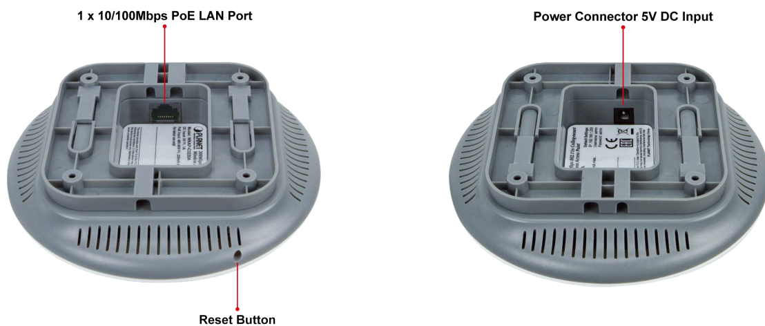
Figure 2-2 WNAP-C3220A Rear Panel
