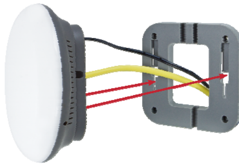
Figure 3-3 WNAP-C3220A Installation Diagram 3
