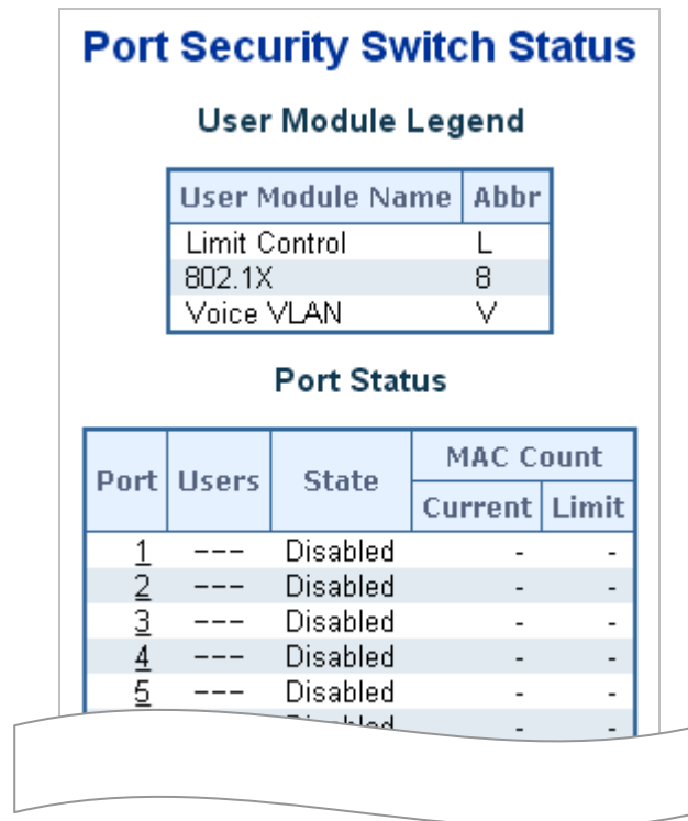
Figure 4-12-6: Port Security Status Screen page Screenshot
