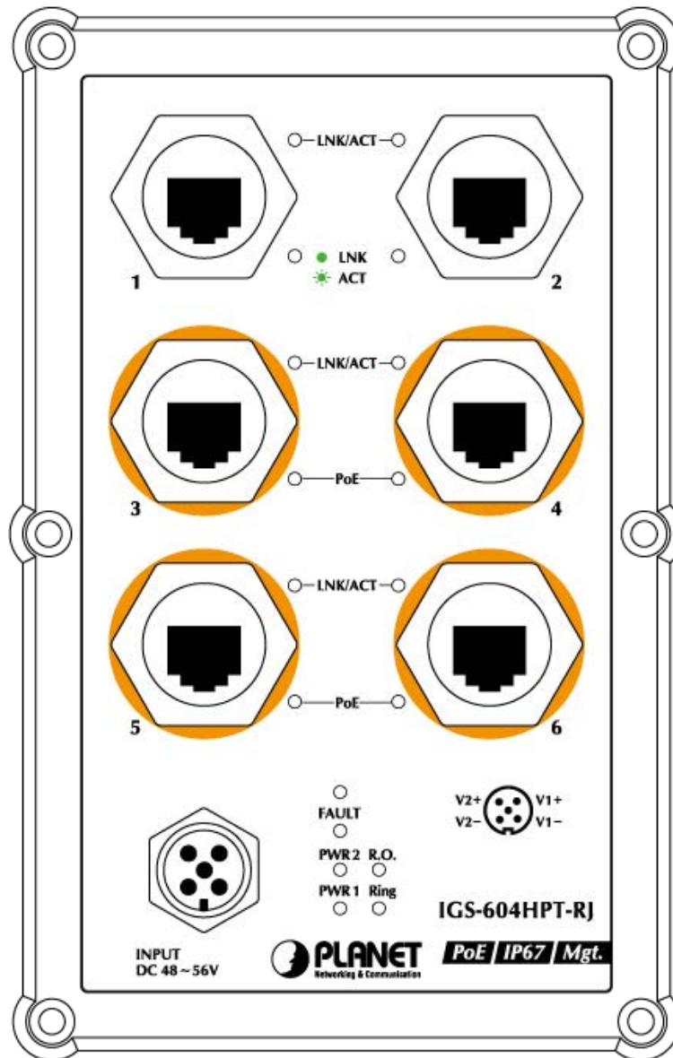
Figure 2-1: IGS-604HPT-RJ Switch Front Panel
