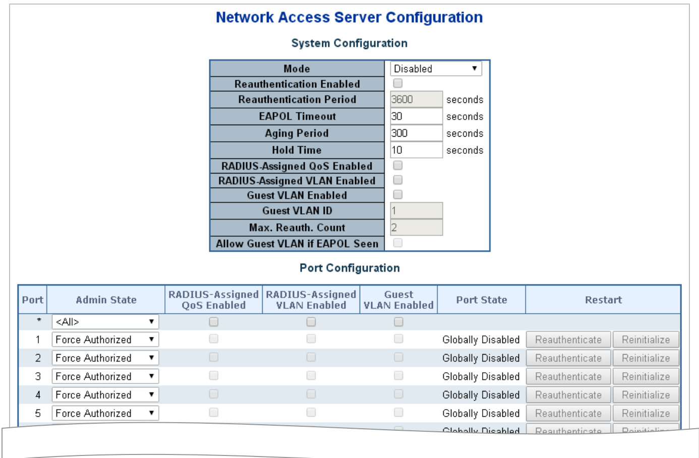
Figure 4-11-4: Network Access Server Configuration page Screenshot
