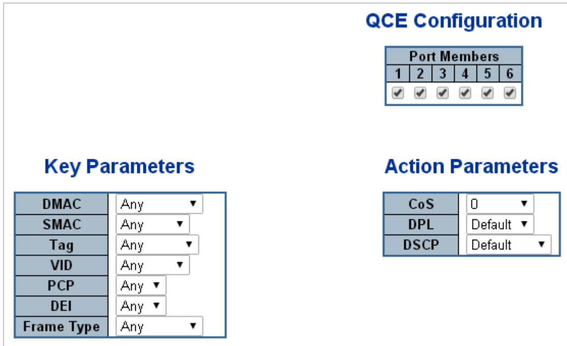
Figure 4-9-13: QCE Configuration page Screenshot
