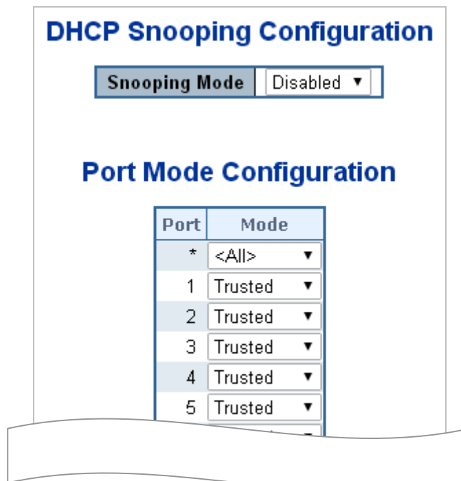
Figure 4-12-8: DHCP Snooping Configuration Screen page Screenshot
