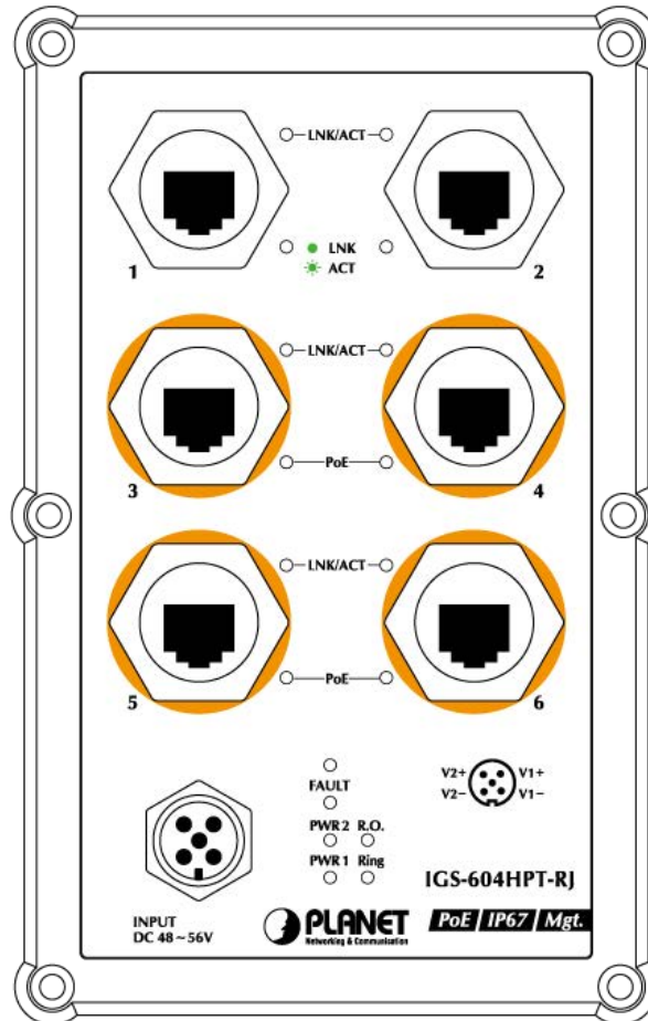
Figure 2-2: IGS-604HPT-RJ LED on Front Panel
