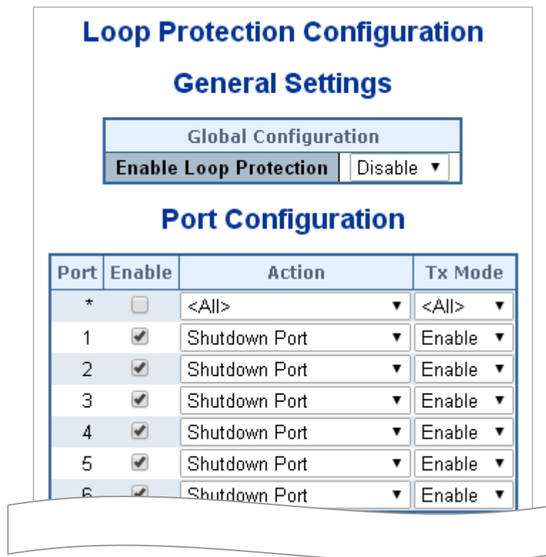
Figure 4-17-1: Loop Protection Configuration page Screenshot
