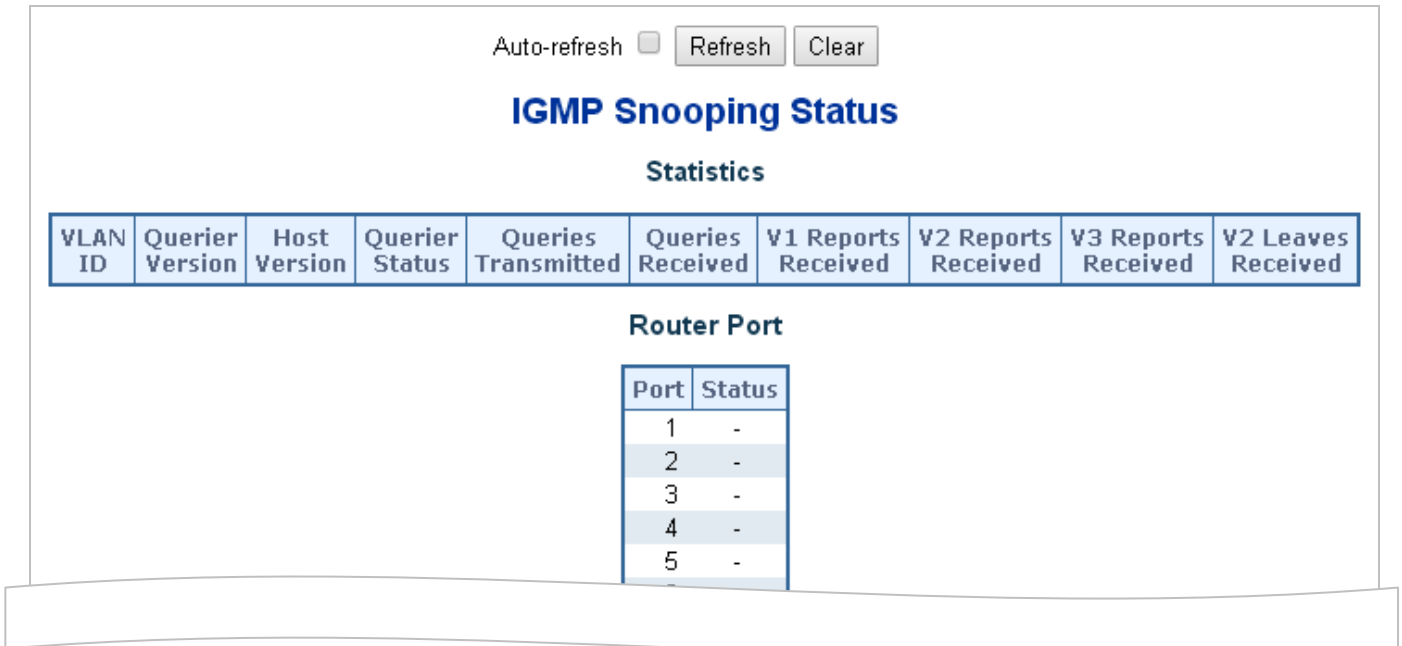
Figure 4-8-10: IGMP Snooping Status page Screenshot
