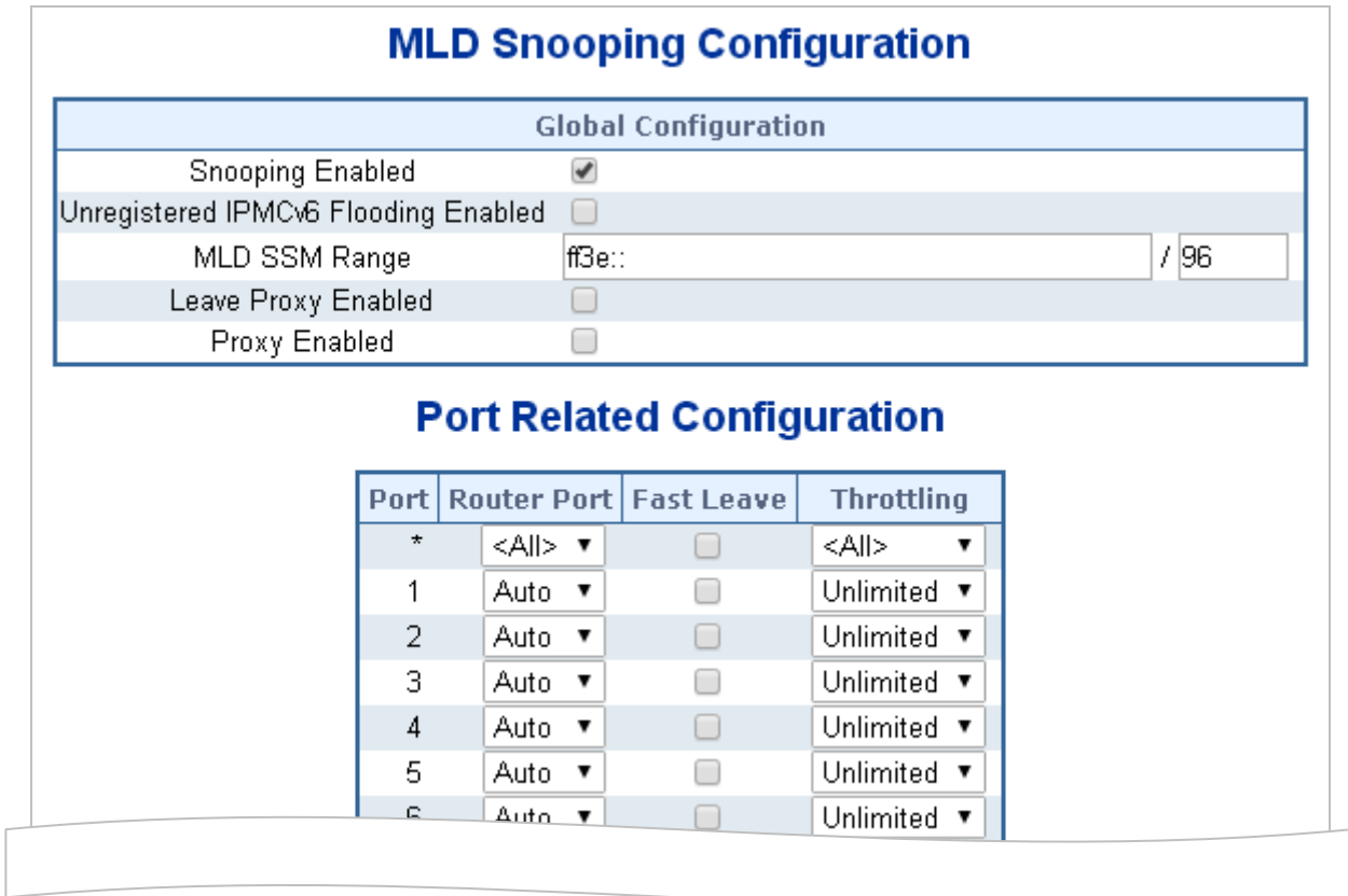
Figure 4-8-13: MLD Snooping Configuration page Screenshot
