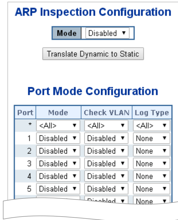
Figure 4-12-13: ARP Inspection Configuration Screen page Screenshot
