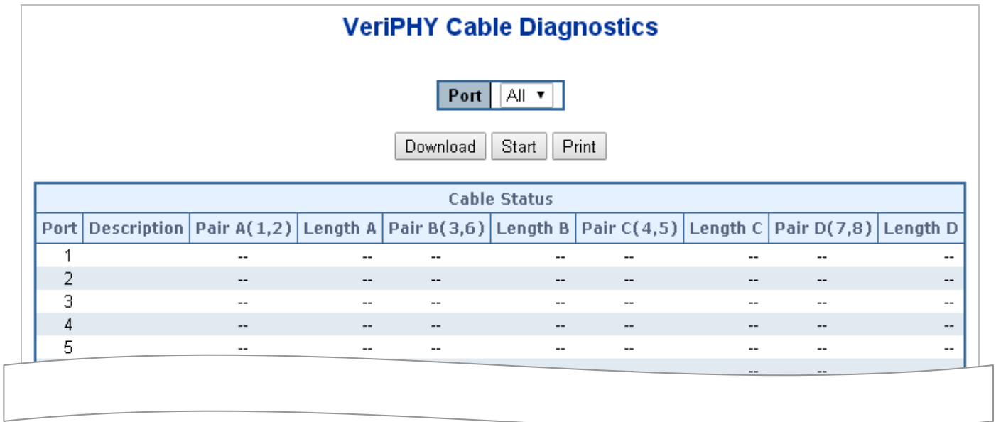
Figure 4-15-4: VeriPHY Cable Diagnostics page Screenshot
