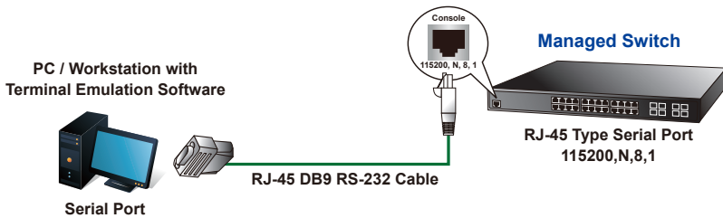
Figure 3-1: Managed Switch Console Connectivity
