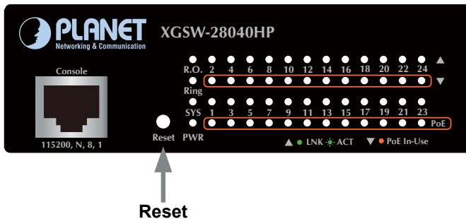
Figure 8-1: XGSW-28040HP Reset Button
