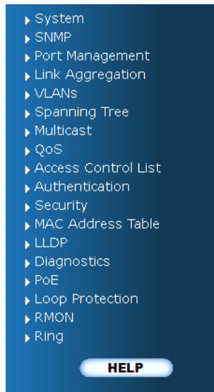
Figure 6-4: Switch Menu
