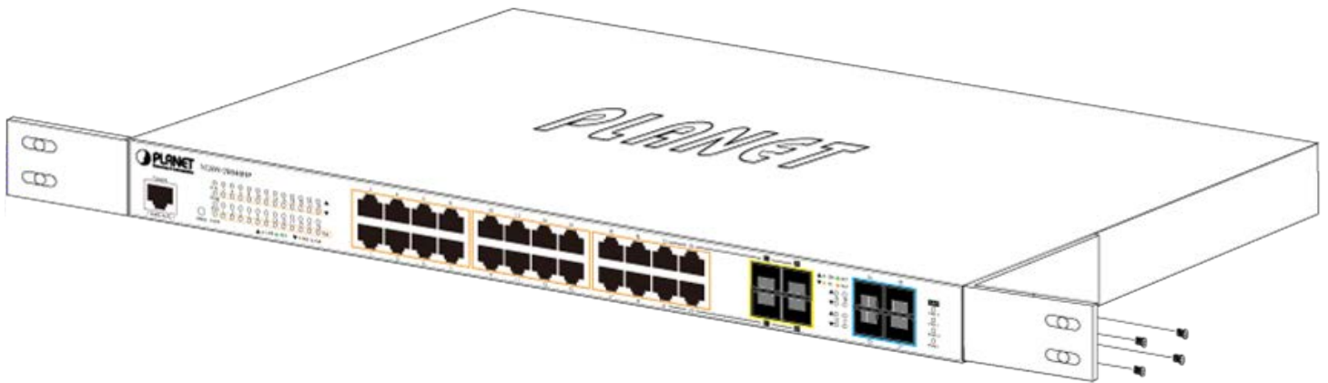
Figure 2-2-2: Attach Brackets to the Managed Switch.
