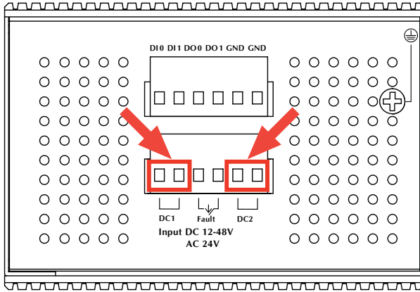
Figure 3-5: IGS-20040MT Upper Panel
