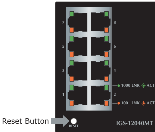
Figure 8-4: IGS-12040MT Reset Button
