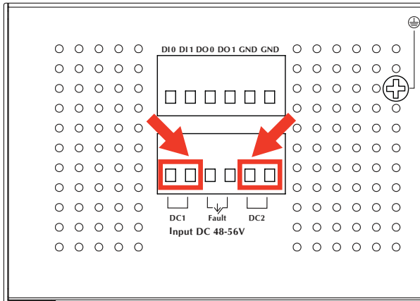
Figure 3-6: IGS-20160HPT Upper Panel
