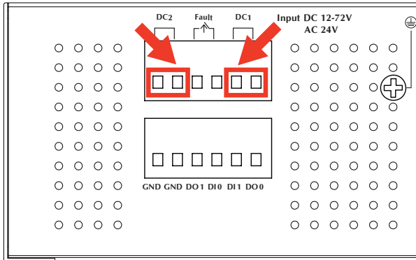
Figure 3-4: IGS-12040MT Upper Panel
