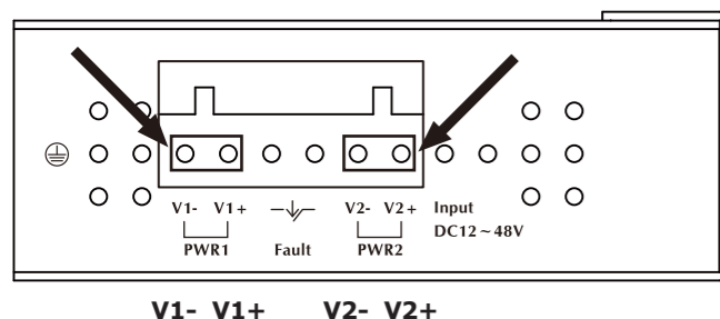
Figure 1 PWR1 & PWR2 of Industrial Serial Converter.
