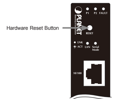
Figure 6 Reset button
